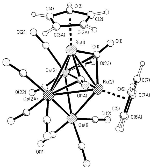
Fig. 3 Molecular structure of [\text{Os}_3\text{Ru}_2(\text{CO})_9(\mu_3\text{-CO})_2(\eta^5\text{-C}_5\text{H}_5)] 5 showing the atom numbering scheme
